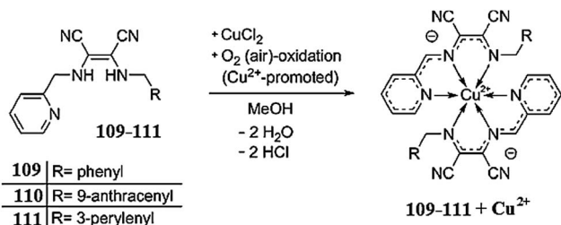
Fig. 94 Chemical structure of receptor 109–111 and selective Cu 2+ -promoted air oxidation and deprotonation in the receptors to form copper complexes.
