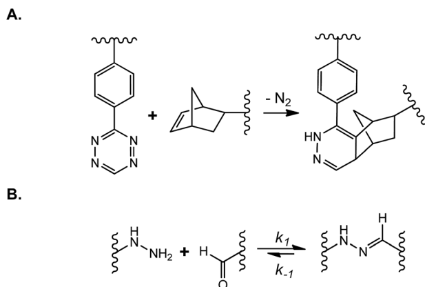
Fig. 8 (A) Tetrazine–norbornene click reaction; (B) covalently adaptable network formed by N -methyl hydrazine–butyaldehyde ligation.
