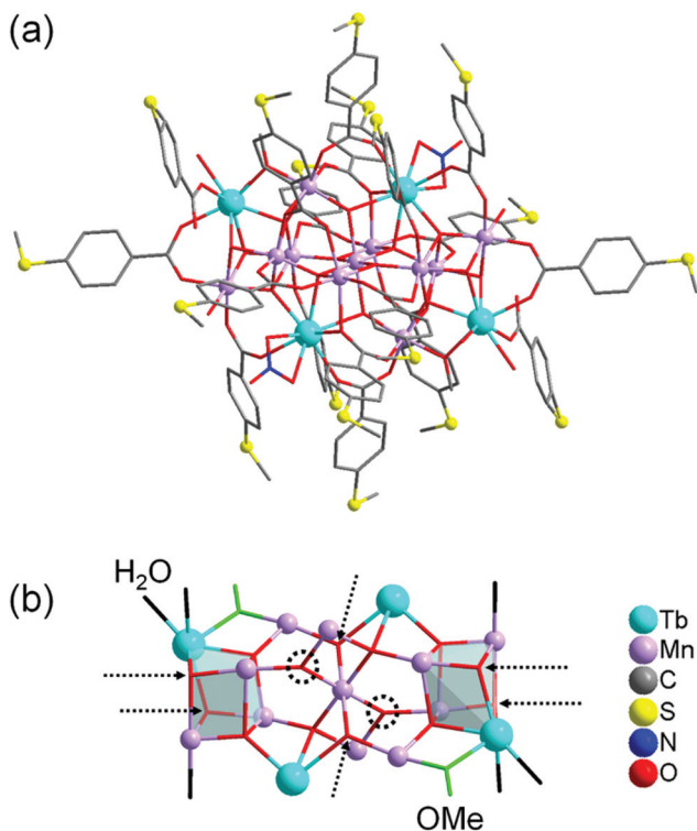
Fig. 1 (a) Molecular structure of compound 1 . (b) Metal–oxide skeleton \{\text{Mn}_{11}\text{Tb}_4\text{O}_{14}\} of compound 1 incorporating two methoxide anions and six water molecules (eighteen \text{bza}\cdot\text{SMe}^- ligands and two \text{NO}_3^- ligands are not shown). Six possible \mu_3\text{-O} protonation sites are indicated by dashed arrows and the two remaining, nonprotonated \mu_3\text{-O} oxygen atoms by dashed circles. Hydrogen atoms are omitted for clarity. The metal and sulfur atoms are represented as ball-and-stick models. Selected bond lengths [Å]: Tb–O (of \text{H}_2\text{O} ) 2.371(10) and 2.427(9), Tb–O (of \text{MeO}^- ) 2.282(8), Tb– \mu_3\text{-O} 2.366(8)–2.492(8), Tb– \mu_4\text{-O} 2.388(7)–2.565(7), Mn–O (of \text{H}_2\text{O} ) 2.212(9), Mn–O (of \text{MeO}^- ) 1.891(8), Mn– \mu_3\text{-O} 1.870(7)–2.300(8), Mn– \mu_4\text{-O} 1.860(7)–2.440(7), nearest-neighbor Mn–Tb 3.4045(18), nearest-neighbor Mn–Mn 2.855(2). All bond lengths and angles are reported in the ESI†
