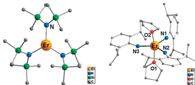
Fig. 6 Molecular structures of the complexes [\text{Er}\{\text{N}(\text{SiMe}_3)_2\}_3] (left) and [\text{Er}\{\text{NHPh}(\text{Pr})_2\}_3(\text{THF})_2] (right), with hydrogen atoms omitted for clarity. Adapted with permission from ref. 22. Copyright 2014 American Chemical Society.
