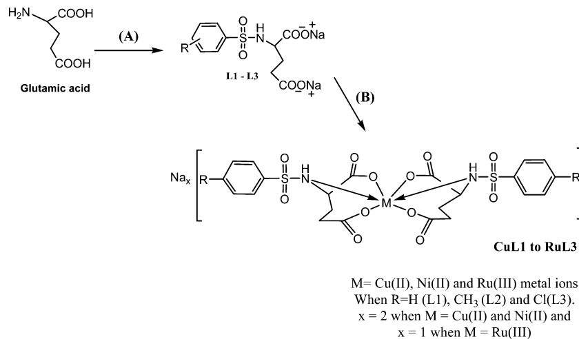
Scheme 2 Schematic depiction of the syntheses of ligands L1–L3 and their complexes (CuL1 to RuL3). Reagents and conditions: (A) solid sodium hydroxide, benzenesulphonyl chlorides, reflux at 70 °C for 8 h, (B) hydrated metal chlorides.
