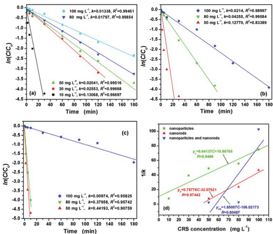
Fig. 7 The effect of initial CRS concentration on the degradation kinetics for 50 mL CR solution at different time intervals: (a) 100 mg \text{CeO}_2 nanoparticles, (b) 20 mg \text{CeO}_2 nanorods, (c) 150 mg \text{CeO}_2 mixture of nanoparticles and nanorods, and (d) the relationship between the degradation rate constant k and CRS concentrations from 10 to 100 \text{mg L}^{-1} .
