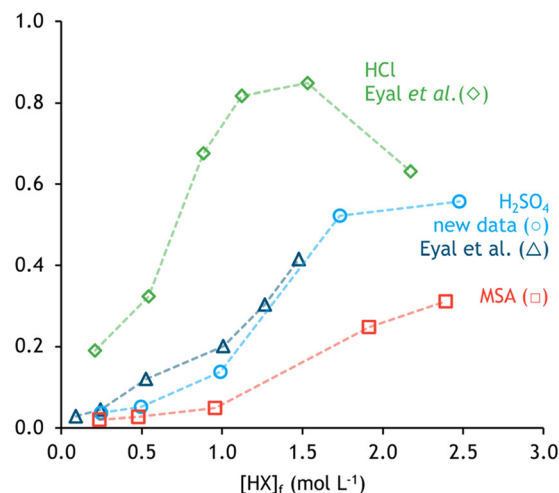
Fig. 3 Solvent extraction data of H_2SO_4 , HCl, and MSA – TEHA + dodecane systems at 25 °C. Graph c compares this to literature data from Eyal et al. 46 Distribution ratios are shown for three TEHA concentrations with varying H_2SO_4 concentrations in the feed (a), and with varying initial TEHA concentrations in the solvent (b). (c) Compares the extraction of HCl, H_2SO_4 , MSA by 43 vol% TEHA.
