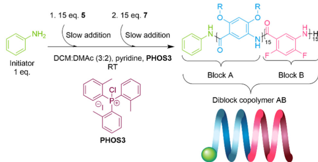
Scheme 2 Top: Synthetic paths for monomers 5 and 7 . (a) K 2 CO 3 , DMF, 15-bromo-2,5,8,11-tetraoxapentadecane 2 , 51%. (b) H 2 /Pd/C, MeOH, EtOAc, quant. (c) KOH, EtOH, 60%. (d) H 2 /Pd/C, MeOH, EtOAc, quant. Bottom: Polymerization conditions of diblock copolymer AB.
