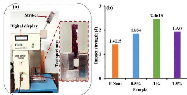
Fig. 7 (a) Impact test setup and (b) impact strength of a tested specimen with varying wt% of G.
