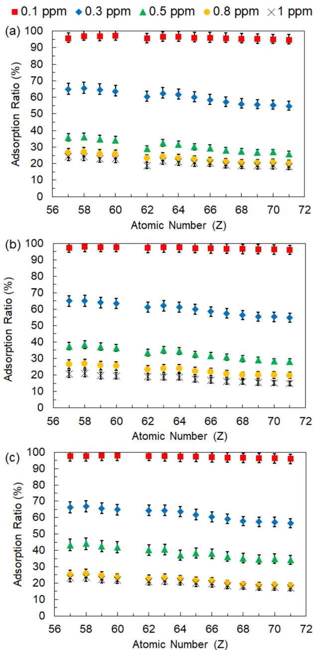
Fig. 6 Adsorption rates of all Ln ions (atomic numbers of 57 to 71 corresponding to La to Lu, respectively) on P-SiO 2 -poly(DMAPS) at temperatures of (a) 50 °C, (b) 60 °C, and (c) 70 °C.
