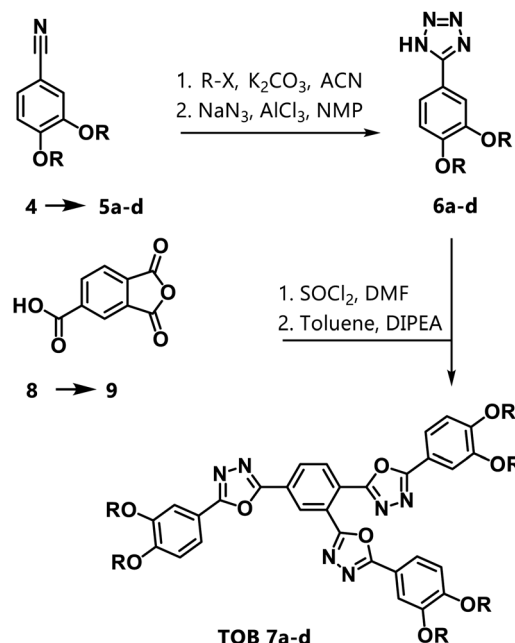
Scheme 1 Synthesis of TOBs . a: R = octyl, b: R = decyl, c: R = dodecyl, d: R = 3,7-dimethyloctyl.
