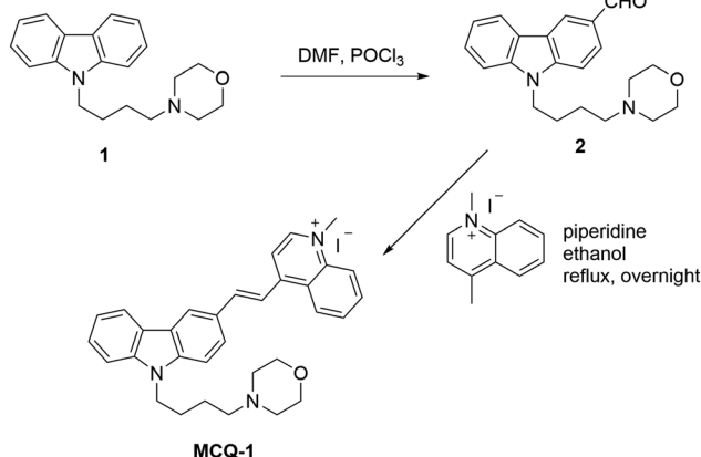
Scheme 1 Synthesis of MCQ-1 .
