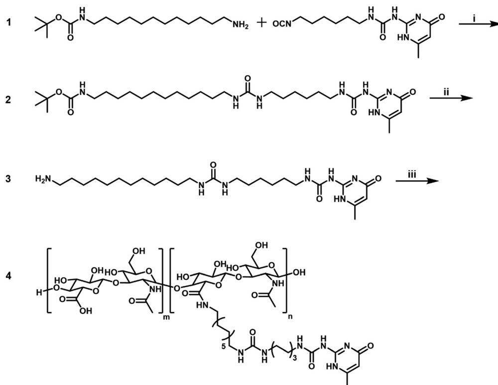
Scheme 1 Synthetic procedure for the functionalization of a hyaluronic acid backbone with UPy-moieties. Reaction conditions: (i) \text{CHCl}_3 , 50 °C, 16 hours, 91% yield; (ii) TFA: DCM 1:1 v/v%, 2.5 hours, yield 101%; (iii) 0.08 eq. hyaluronic acid, 1.1 eq. PyBOP, 23.3 eq. TEA, DMSO, r.t., 16 hours, 53% yield.
