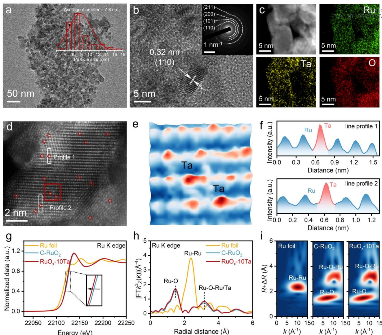
Fig. 1 Structural characterization of RuO x -αTa. (a) TEM image with diameter distribution (inset) of the RuO x -10Ta. (b) HR-TEM image of RuO x -10Ta with SAED image (inset). (c) Elemental mappings of RuO x -10Ta. (d) Aberration-corrected HAADF-STEM image. (e) 3D atom-overlapping Gaussian function fitting mapping of the selected red squares area in (d). (f) Intensity profiles along the yellow rectangle regions in (d). (g) Ru K-edge XANES spectra of RuO x -10Ta and the corresponding reference samples. (h) Fourier transforms of k^3 -weighted spectra at Ru K edge of RuO x -10Ta and the corresponding reference samples. (i) Wavelet transform for k^3 -weighted EXAFS signals at the Ru K-edge of RuO x -10Ta and the corresponding reference samples.
