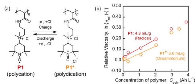
Fig. 2 (a) Redox reaction of the TEMPO moiety in P1 to yield the polydication P1 + bearing the oxoammonium moiety per repeating unit. (b) Concentration dependence of the viscosity of the poly-electrolytes in the charged state P1 + (◇) and the discharged state P1 (○).
