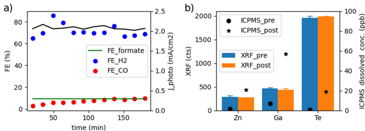
Fig. 10 (a) Stability test of ZnGa 2 Te 4 without additives using a traditional H-cell at -0.8 V vs. RHE with periodic headspace measurements. Note that formate shown in the figure is the average over entire measurement. (b) Corrosion study by ICP-MS and XRF for pre- and post-PEC run samples.
