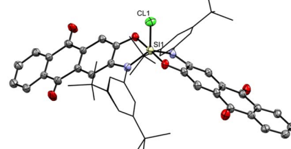
Fig. 5 (a) Synthesis of pentacoordinate silicon complexes with neutral and anionic donors. (b) Molecular structure of [\mathbf{1-Cl}][\text{PPh}_4] determined by SCXRD analysis. Hydrogen atoms and the \text{PPh}_4 cation are omitted for clarity. Thermal displacement ellipsoids are displayed at the 50% probability level. Selected bond lengths [pm]: Si1–Cl1: 211.64(10), Si1–O1: 174.78(18), Si1–N1: 178.1(2). Selected bond angles [°]: N1–Si1–N1: 128.16(10), O1–Si1–O4: 177.74(9), N1–Si1–Cl1: 116.45(8), O1–Si1–Cl1: 91.53(7).
