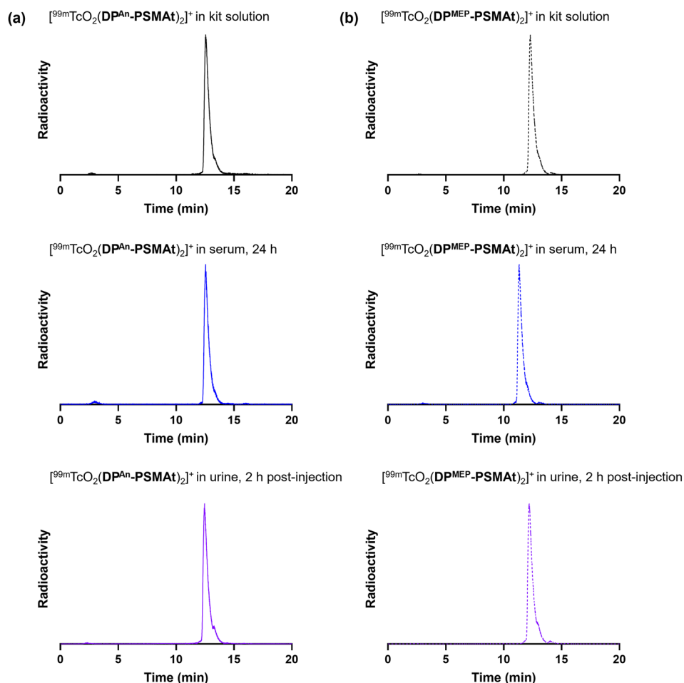
Fig. 3 Radiochromatograms of reactions containing (a) ^{99m}\text{TcO}_2(\text{DP}^{\text{An}}\text{-PSMA})_2]^+ and (b) ^{99m}\text{TcO}_2(\text{DP}^{\text{MEP}}\text{-PSMA})_2]^+ , including radiochromatograms of ^{99m}\text{Tc} samples after either incubation in human serum at 37 ^\circ\text{C} , or after administration to a mouse, followed by collection of urine 2 hours post-administration. Radio-HPLC analyses of serum and urine samples indicate that ^{99m}\text{Tc} radiotracers possess high stability in the presence of serum proteins and in vivo .
