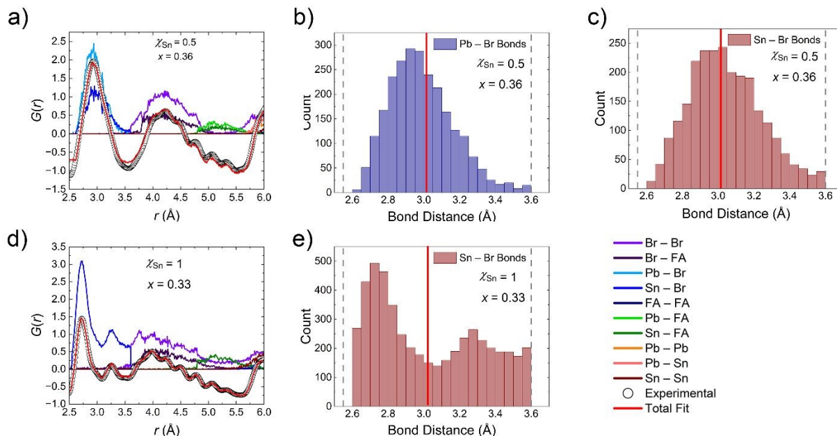
Figure 9: Results from Reverse Monte Carlo fitting of the low r region (2.5 – 6 Å) of the experimental PDF curve for \text{FA}_{0.64}\text{en}_{0.36}\text{Pb}_{0.42}\text{Sn}_{0.40}\text{Br}_3 (a) and histogram of the Pb – Br (b) and Sn – Br (c) bond distances extracted from the resulting model as well as the corresponding plots for \text{FA}_{0.67}\text{en}_{0.33}\text{Sn}_{0.84}\text{Br}_3 (d and e). The average bond distance determined from single crystal X-ray diffraction are displayed as a red lines on the histograms.
