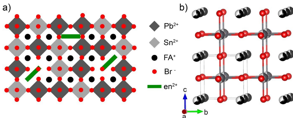
Figure 6: a) a depiction of the ethylenediammonium substitutions into the metal halide perovskite lattice and b) a representative average crystal structure for the \text{FA}_{1-x}\text{en}_x\text{Pb}_{1-y}\text{Sn}_y\text{Br}_3 family of hollow perovskites. The atoms are shown in grey, silver, red, black, and white for Pb, Sn, Br, \text{FA}^+ , and vacancies respectively.
