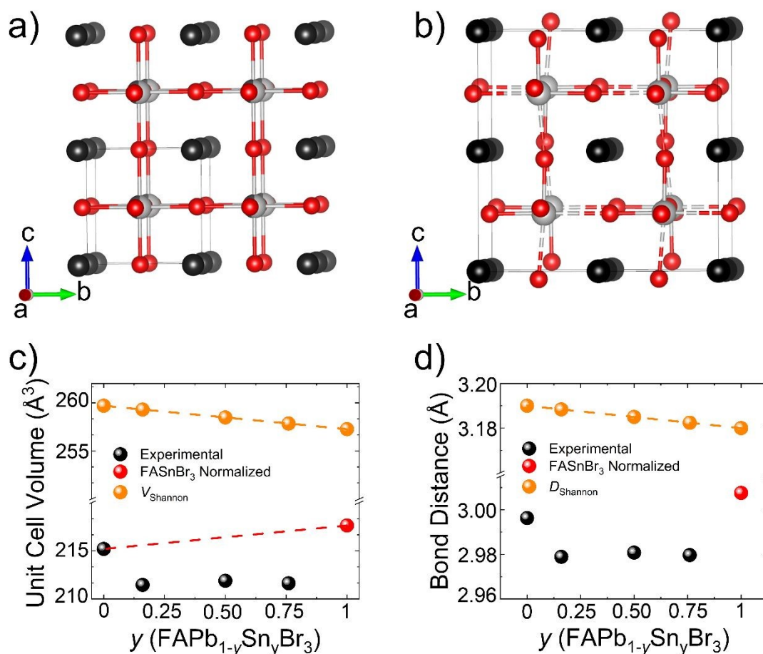
Figure 5: a) the overall structure for \text{FAPb}_{0.5}\text{Sn}_{0.5}\text{Br}_3 and b) \text{FASnBr}_3 as displayed down the crystallographic a -axis, c) the trend in the experimental unit cell volume compared to the theoretical Shannon volume as a function of Sn content, and d) the trend in bond distance compared to the predicted Shannon distance as a function of Sn content. The atoms are shown in grey, silver, red, and black for Pb, Sn, Br, and \text{FA}^+ respectively.
