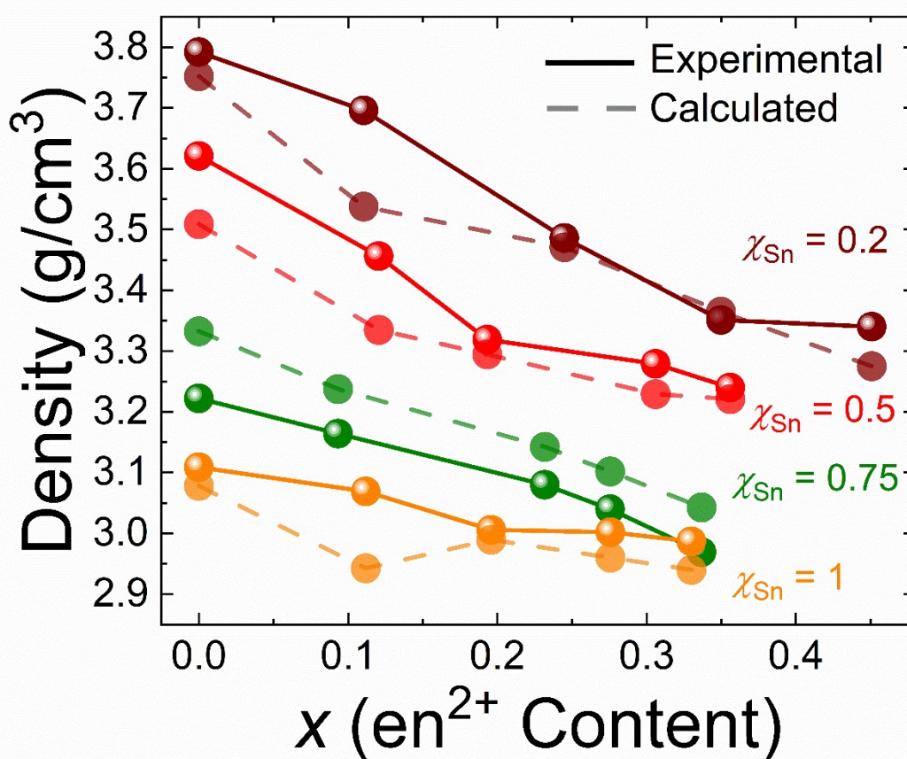
Figure 4: Experimental and calculated density ( \text{g/cm}^3 ) from single crystal refinements for each material plotted as a function of ethylenediammonium ( \text{en}^{2+} ) substitution. The experimental and calculated densities are represented by solid and dashed lines, respectively.
