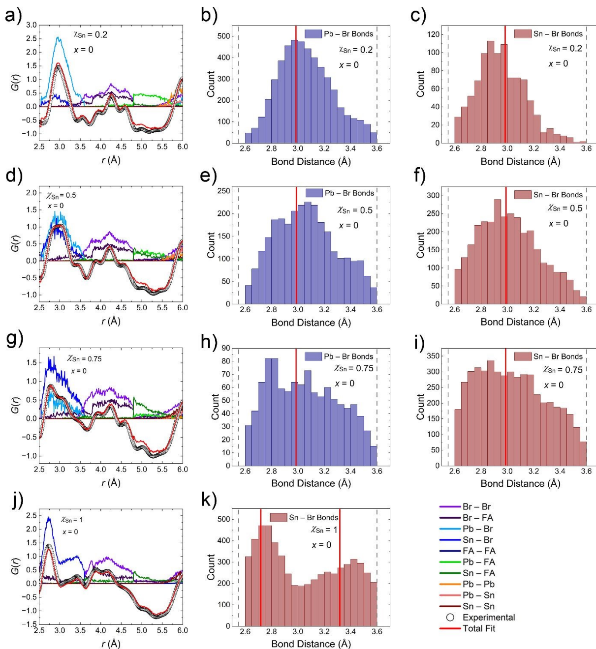
Figure 8: Results from Reverse Monte Carlo fitting of the low r region (2.5 – 6 Å) of the experimental PDF curves for the \text{FAPb}_{1-y}\text{Sn}_y\text{Br}_3 ( y = 0.2, 0.5, 0.75, 1 ) compounds (a, d, g, j) and histograms of the Pb-Br (b, e, h) and Sn-Br (c, f, i, k) bond distances extracted from the resulting model. The average bond distance(s) determined from single crystal X-ray diffraction are displayed as red line(s) on the histograms.
