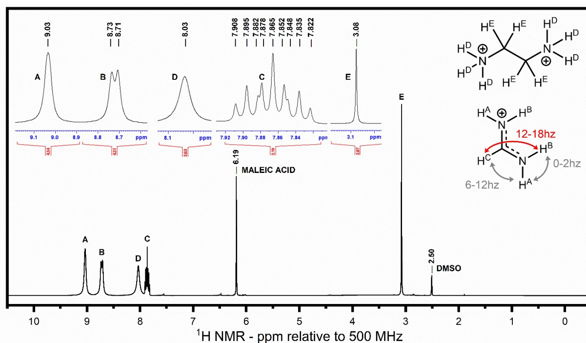
Figure 2: ^1\text{H} NMR (500 MHz, \text{DMSO-d}_6 = 2.50 ) \delta 9.03 (br s, 2H, A, FA exo NH), 8.72 (br d, J = 13.8 Hz, 2H, B, FA endo NH), 8.03 (br s, 3H, D, EN \text{NH}_3 ), 7.86 (dddd, J = 14.9, 14.9, 6.4, 6.4 Hz, 1H, C, FA CH), 3.08 (s, 4H, E, EN (\text{CH}_2)_2 ; dddd = doublet of doublets of doublets of doublets)
