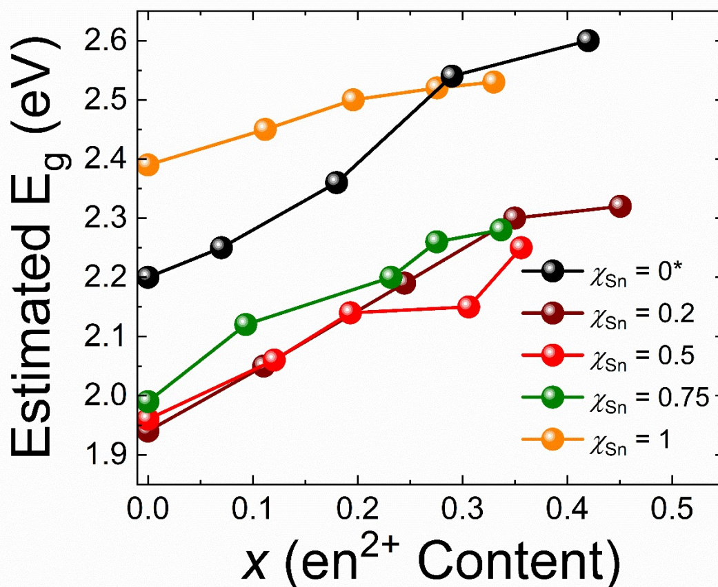
Figure 10: Depicts the trend in estimated E_g (eV) as a function of the experimentally determined ethylenediammonium content. *The \chi_{\text{Sn}} = 0 line is plotted based on data from our previous works. 38
