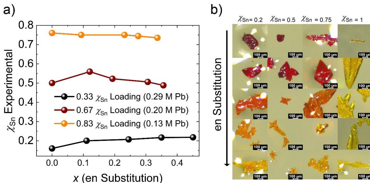
Figure 1: a) Depicts the mol fraction of Sn ( \chi_{\text{Sn}}^{\text{Experimental}} ), determined by ICP-OES, as a function of ethylenediammonium substitution ( x ) in the \text{FA}_{1-x}\text{en}_x\text{Pb}_y\text{Sn}_{1-y}\text{Br}_3 family. The mol fraction of Sn charged to the reaction solution ( \chi_{\text{Sn}}^{\text{Loading}} ) is also labeled with the corresponding \text{Sn}^{2+} reaction concentration in mol/L determined from the synthetic conditions (see the supporting information). b) A selection of crystal images to illustrate typical crystal morphologies and colors. The representative experimental Sn fraction is labeled for each column of crystals.
