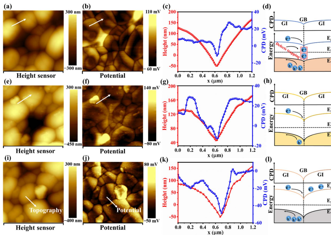
Fig. 4 KPFM scanning surface topography and CPD maps for (a and b) Sb 2 Se 3 , (e and f) Sb 2 Se 3 /CdS, and (i and j) Sb 2 Se 3 /CdS/MoS 2 samples, respectively. (c, g and k) The corresponding topography and potential line scans acquired from the white arrow lines. (d, h and l) Schematic of the energy band structure and CPD near the GBs, where “e - ” represents electrons; “h + ” represents holes.
