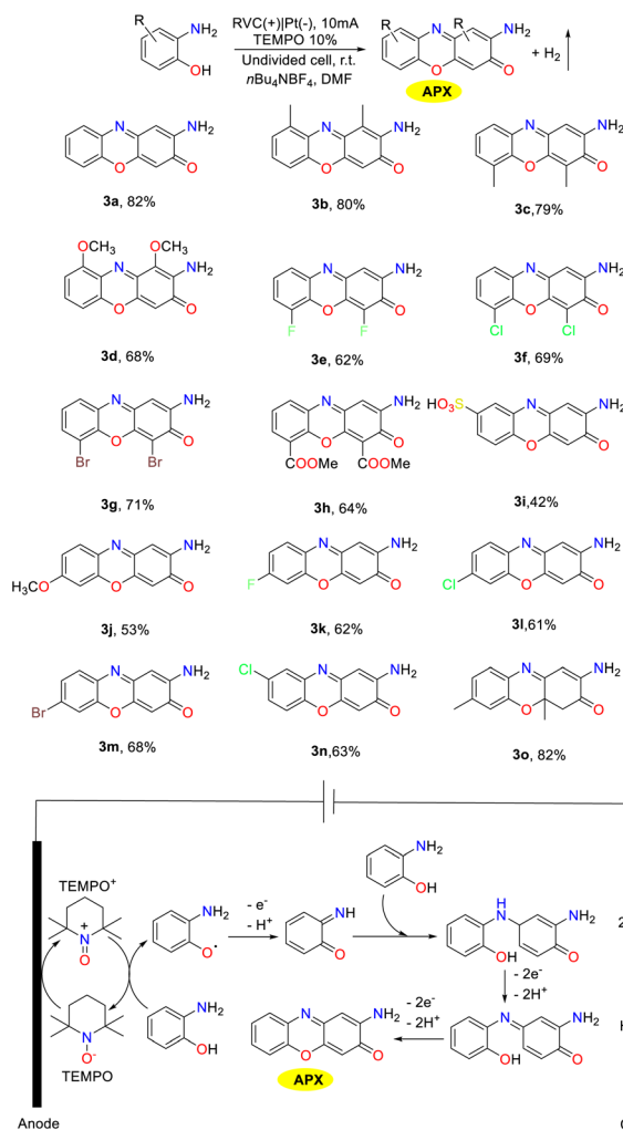
Scheme 61 Electrochemical dehydrogenative cyclocondensation of o -aminophenols (ref. 21).
