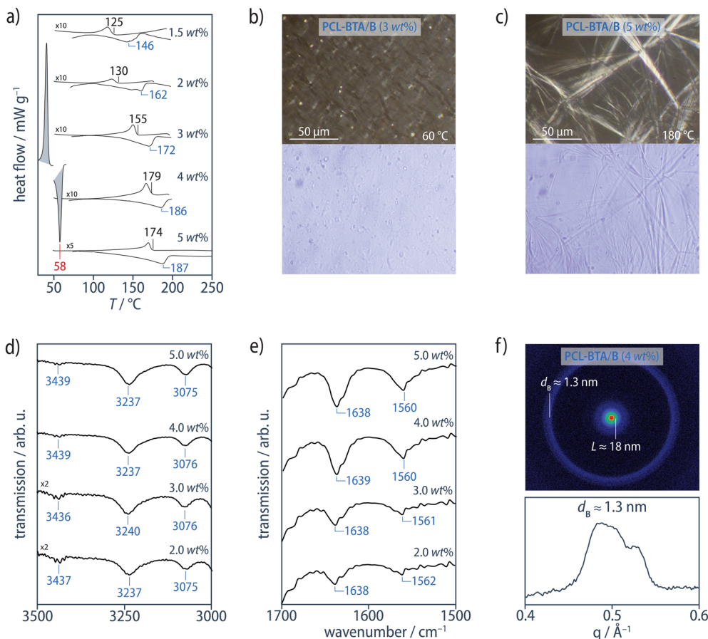
Fig. 4 (a) DSC heating and cooling scans (10 °C min -1 , exothermal transitions up) from the PCL-BTA/B blends for B concentrations \geq 1.5 wt%. For clarity, the PCL melting and crystallization transitions at T_m = 58 °C and T_c = 35 °C, respectively, are only shown for one composition. (b and c) Cross-polarized (top) and bright-field (bottom) optical micrographs of PCL-BTA/B recorded at T < T_{agg} during cooling at 10 °C min -1 from the melt state. PCL-BTA/B blends containing \geq 1.5 wt% B show microfibrous precipitates (see also ESI Fig. S12†). (d) The N-H stretching band, and (e) the C=O stretching band and the combined N-H bending/C-N stretching band from ATR FTIR spectra of PCL-BTA/B recorded at 25 °C. The sharp absorption signal visible in all the spectra at 3435–3445 cm -1 is assigned to water absorbed by PCL. 92 (f) The corresponding structures show Bragg reflections in the neighborhood of q \approx 0.24 Å -1 ( d_B \approx 1.3 nm) in XRD patterns obtained at room temperature.
