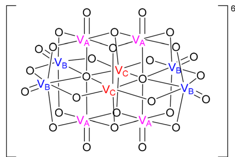
Fig. 2 \text{V}_A , \text{V}_B , and \text{V}_C centres in [\text{V}_{10}^{\text{VO}}\text{O}_{28}]^{6-} .
