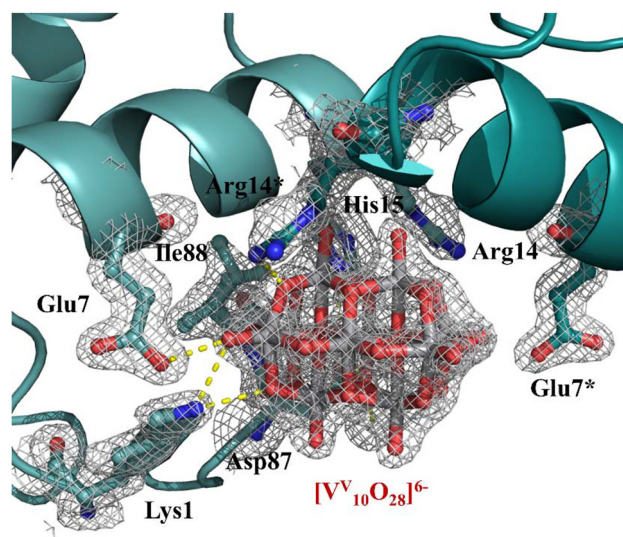
Fig. 9 Vanadium binding sites in structure B: non-covalent interaction of the [V_{10}O_{28}]^{6-} to the protein surface. 2Fo-Fc electron density maps are reported at 1.0σ level in grey. Asterisk refers to atoms from symmetry-related molecules (deep teal). Anomalous difference electron density map is reported in Fig. S4B.†
