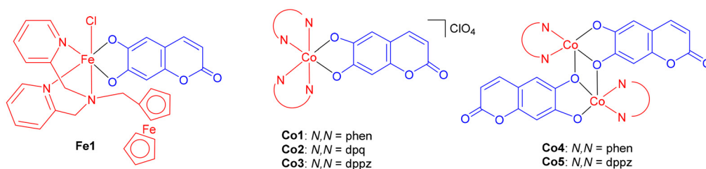
Fig. 10 Earth-abundant metal PSs with coumarin directly coordinated as O^{2-} ligand.
