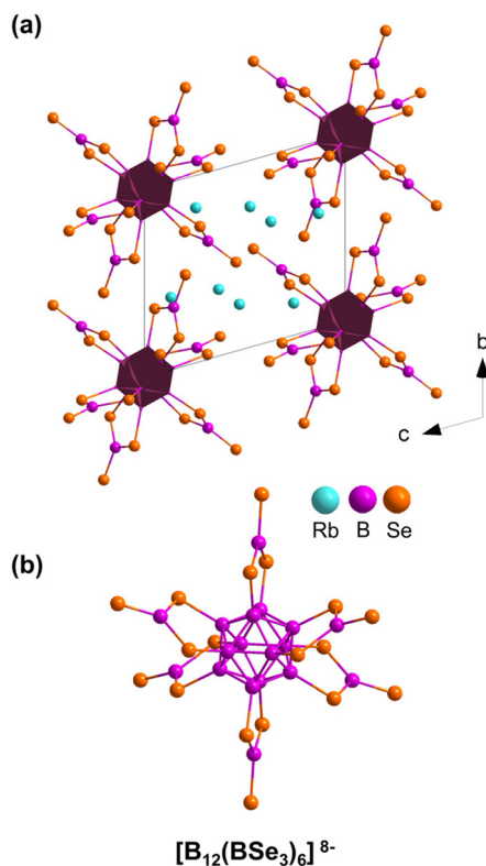
Fig. 12 The structures of (a) the \text{Rb}_8[\text{B}_{12}(\text{BSe}_3)_6] and (b) the [\text{B}_{12}(\text{BSe}_3)_6]^{8-} unit.
