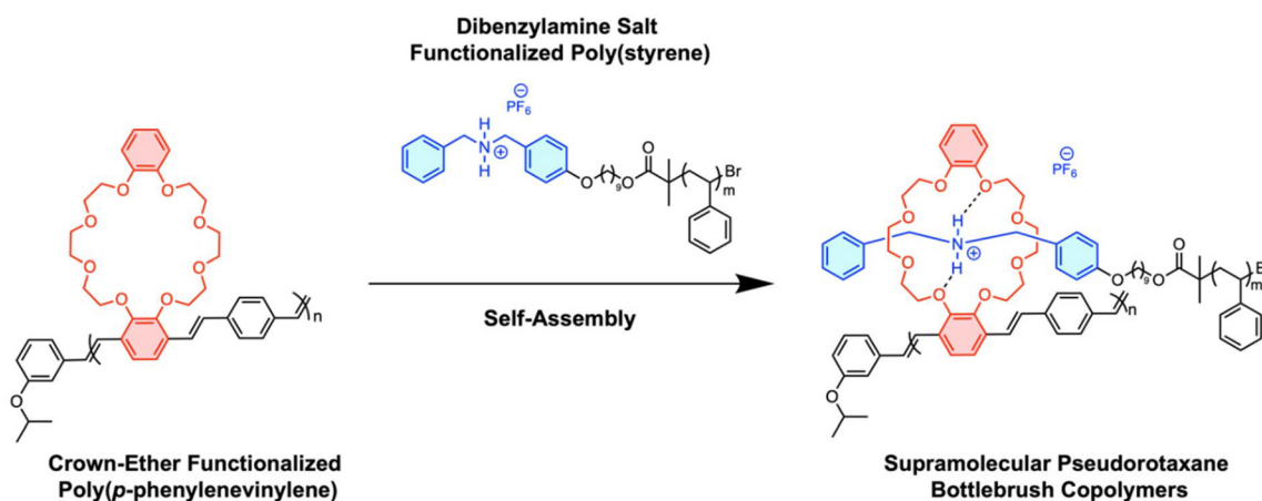
Scheme 2 Synthesis of supramolecular bottlebrush copolymers based on host-guest interactions between crown-ether functionalized poly( p -phenylenevinylene) and dibenzy amine end-functionalized poly(styrene).
