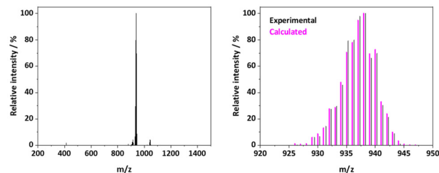
Fig. 1 ESI + spectra (left) and enlargement of the [\text{M}]^+ base peak (right) of RuapNCS .
