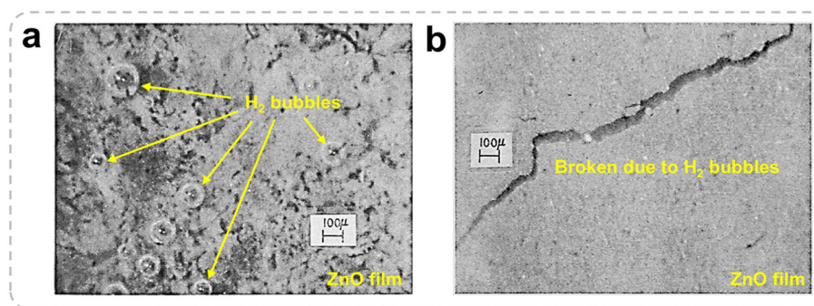
Fig. 9 (a) Hydrogen bubble emergence from the ZnO film. (b) Crack in the ZnO film due to hydrogen bubbles. Reproduced from ref. 47 with permission from IOP Science, copyright 1971.
