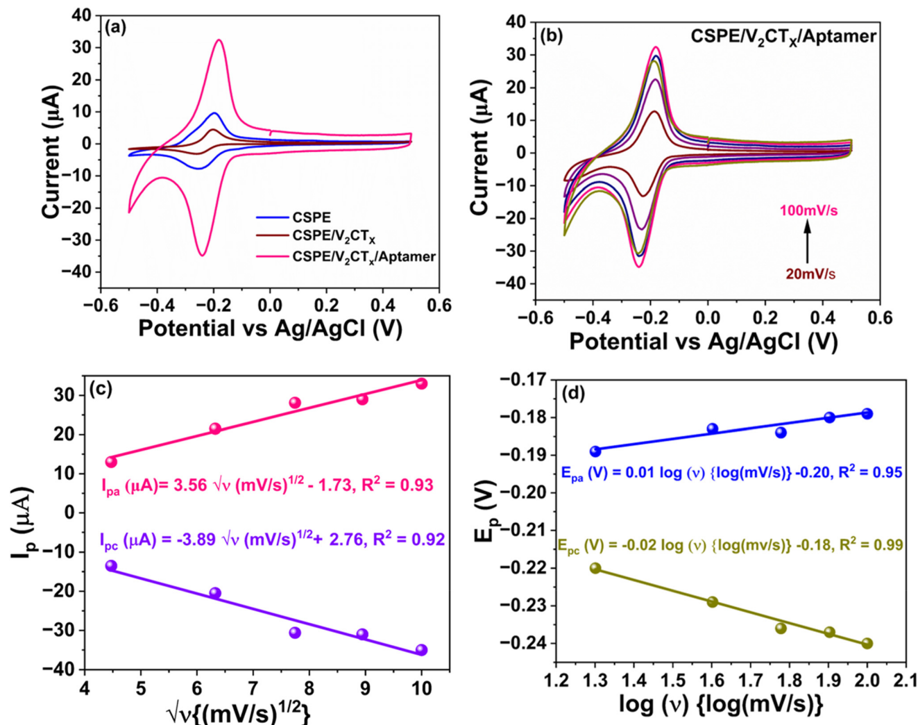
Fig. 3 (a) Cyclic voltammetric response within the potential range of -0.5 to +0.5 V in phosphate-buffered saline/methylene blue at a concentration of 0.1 \text{ M}/1 \mu\text{M} , pH 7, comparing pristine carbon, \text{V}_2\text{CT}_x (2D) and aptamer-coated electrode surfaces. (b) Impact of scan rate on interface current at CSPE/ \text{V}_2\text{CT}_x /aptamer, (c) correlation between the variation of peak current and the square root of scan rate at CSPE/ \text{V}_2\text{CT}_x /aptamer, and (d) impact of scan rate on the redox peak potentials of CSPE/ \text{V}_2\text{CT}_x /aptamer nanoelectrodes.
