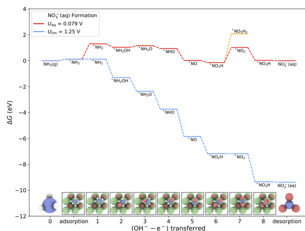
Fig. 14 Free energy diagram for NO_3^-(aq) formation by proceeding through the same mechanistic steps towards NO_2^-(aq) . After *NO_2H is formed, the mechanism branches towards *NO_2 or *NO_3H_2 , with the deprotonation step being energetically preferred. The energy required for the final desorption step was calculated to be -0.029 eV. Equilibrium (red trace) and limiting (blue trace) potentials are calculated using the computational hydrogen electrode at pH 11.
