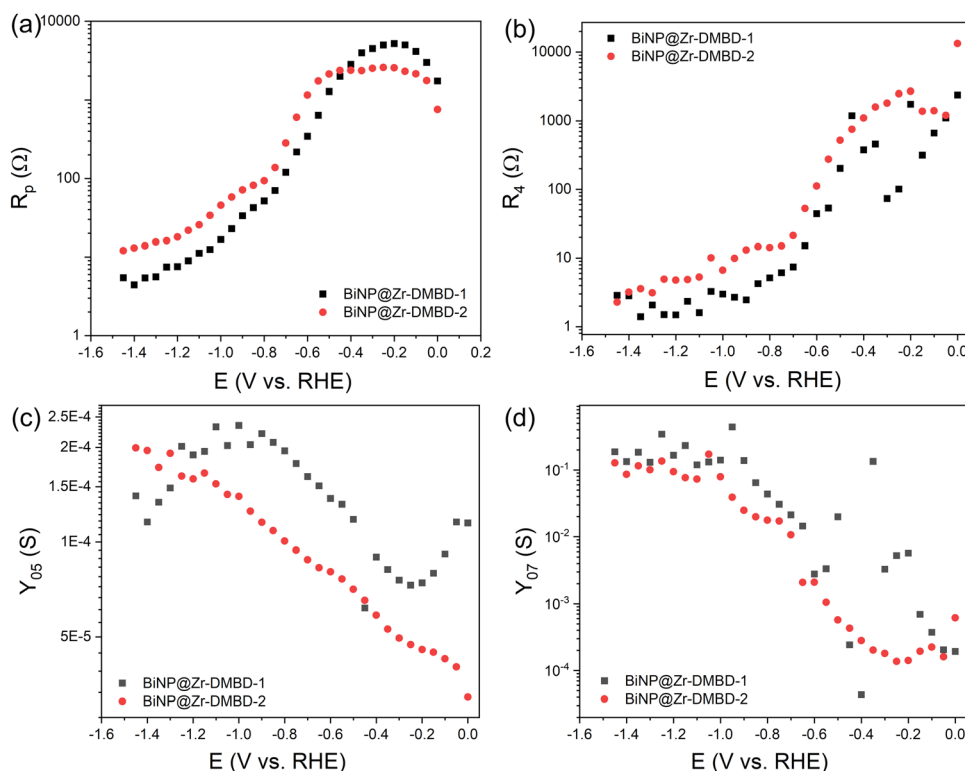
Fig. 6 Charge transfer resistance comparison between BiNP-Zr-DMBD-1 and BiNP-Zr-DMBD-2 at (a) intermediate frequency of 10 Hz to 1 kHz ( R_p ) and (b) low frequency of <1 Hz ( R_4 ). Admittance comparison of the representative pseudocapacitance element at (c) intermediate frequency of 10 Hz to 1 kHz ( Y_{05} ) and (d) low frequency of <1 Hz ( Y_{07} ). EIS fitting was done using modified Armstrong equivalent circuit for multi-step reaction of one adsorbed intermediate. More details are available in ESI†
