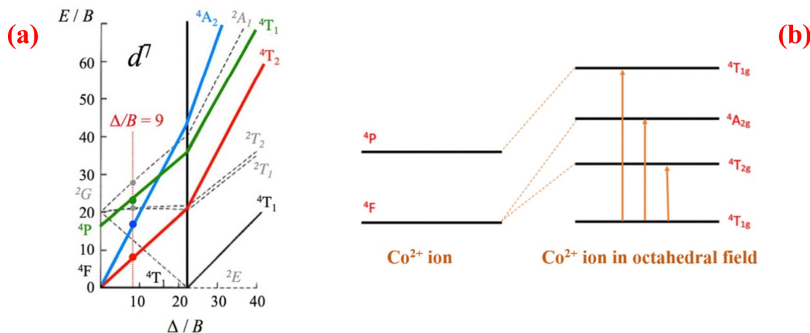
Fig. 3 (a) Simplified Tanabe–Sugano diagram for octahedral \text{Co}^{2+} ( 3d^7 ) 37 (b) The energy levels of the \text{Co}^{2+} ( 3d^7 ) ion in an octahedral field with three spin allowed electronic transitions from d to d in \text{CoO}_6 .
