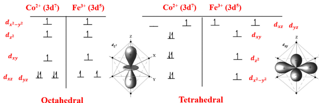
Fig. 4 Crystal field splitting of \text{Fe}^{3+} and \text{Co}^{2+} cation 3d orbitals for tetrahedral and octahedral symmetries. Net spins have been illustrated for every conceivable cation-charge state.
