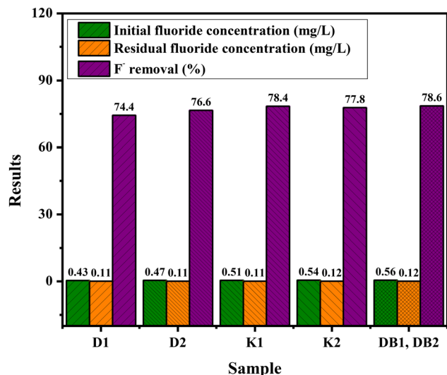
Fig. 16 Water quality analysis of MPVA/1BXT:2AC in Dako, Kuseli and Dabo boreholes.
