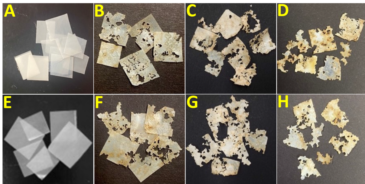
Fig. 1 PCL non-pretreated day 0 (A), day 6 (B), day 12 (C), day 18 (D) and PCL pretreated day 0 (E), day 6 (F), day 12 (G), day 18 (H) in compost. Note: Initial samples were cut to an area of \sim 1 cm 2 .
