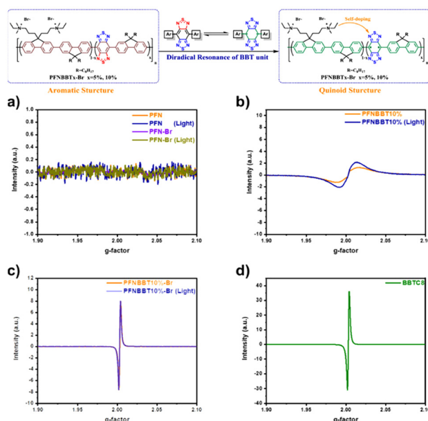
Fig. 11 The ESR spectra of the (a) PFN and PFN-Br, (b) PFNBTT, (c) PFNBTT10%-Br and (d) BBT08.
