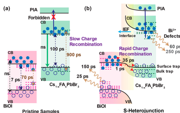
Fig. 6 (a) Depiction of kinetic models for (a) pristine BiOI and \text{Cs}_{1-x}\text{FA}_x\text{PbBr}_3 (CF) and (b) hybrid \text{Cs}_{1-x}\text{FA}_x\text{PbBr}_3 :BiOI (CF:BiOI) heterojunction samples. IEF represents the internal electric field generated in the heterojunction. Reprinted with permission from ref. 106. Copyright 2022, American Chemical Society.
