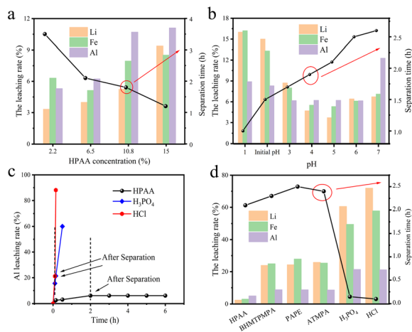
Fig. 2 (a) The concentration and (b) pH of HPAA aqueous solution on the separation efficiency and metal leaching rate. (c) Time-dependent leaching rates of Al in HPAA, HCl and \text{H}_3\text{PO}_4 . (d) Comparison of different agents on the delamination of spent \text{LiFePO}_4 cathodes.
