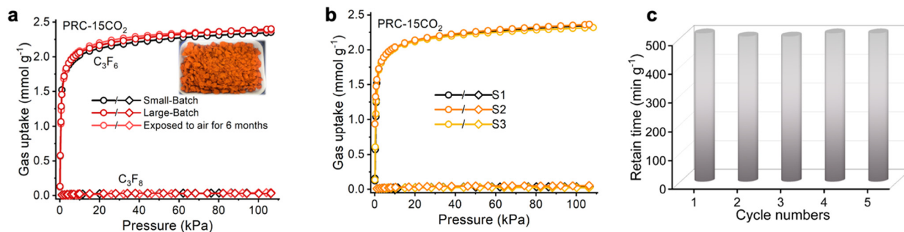
Fig. 5 (a) Comparison of the adsorption isotherms for C_3F_6 and C_3F_8 at 298 K on PRC-15CO 2 synthesized under varying conditions; (b) adsorption isotherms of C_3F_6 and C_3F_8 at 298 K on phenolic resin-derived carbon molecular sieve materials synthesized across different batches; (c) multicycle dynamic breakthrough curves of C_3F_6/C_3F_8 (1/99, v/v) gas mixtures using a packed column bed with PRC-15CO 2 at 298 K and 100 kPa, illustrating the retention times over five dynamic cycles.
