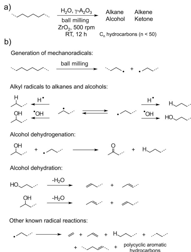
Scheme 6 (a) Mechanochemical degradation of PE by water activation in the presence of \gamma -Al 2 O 3 dispersants. (b) Proposed reaction mechanism involves the generation of alkyl radicals by ball milling and subsequent homolytic water splitting to produce alkanes, alcohols, alkenes and ketones. 66
