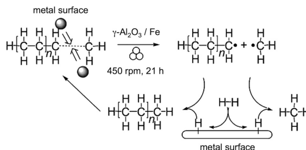
Scheme 5 Mechanochemical gasification of the PE and PET substrates with hydrogen gas in the presence of \gamma -Al 2 O 3 /Fe catalysts. The reaction proceeds by a radical mechanism. 65
