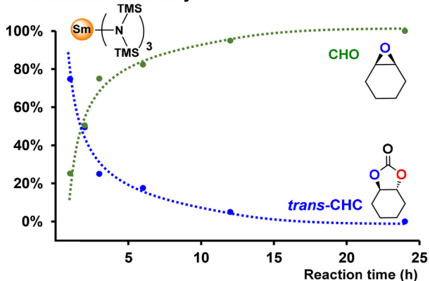
Fig. 1 A. Kinetic profile of PCHC depolymerization in a closed reaction system using \text{La}^{\text{NTMS}} under the conditions of Table 1. B. Total monomer conversion ( trans -CHC + CHO) versus reaction time. C. Kinetic profile of PCHC depolymerization in a closed reaction system using \text{Sm}^{\text{NTMS}} .
