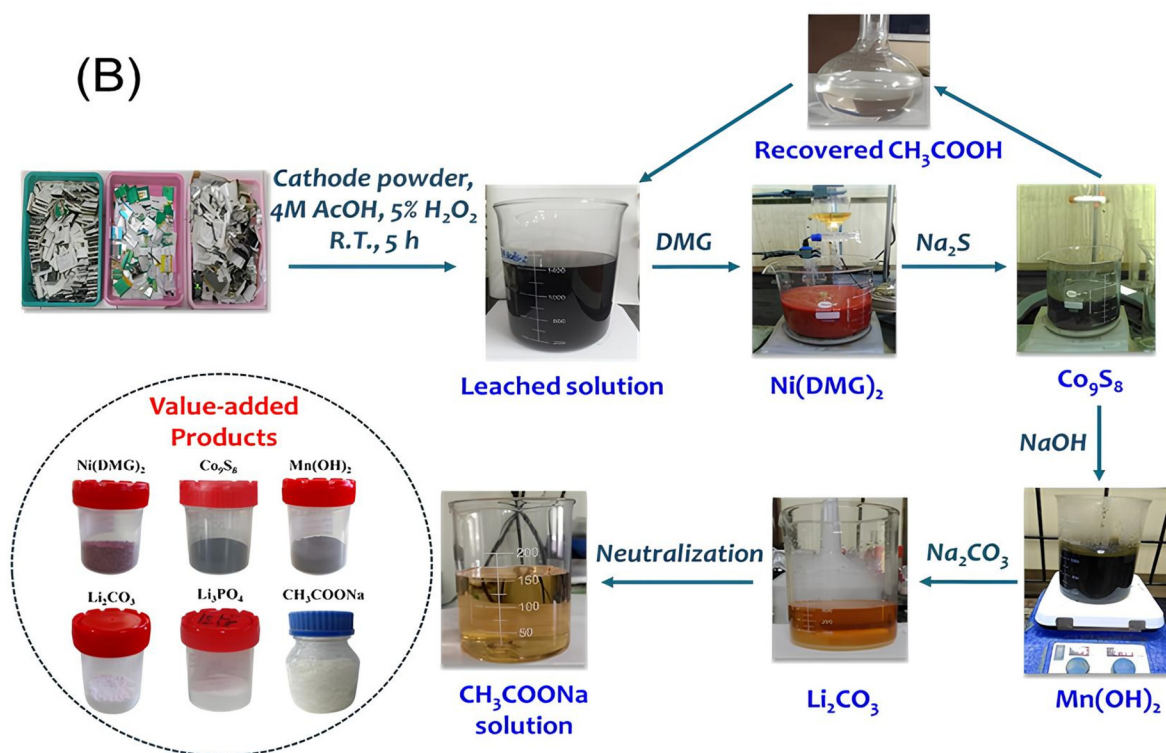
Fig. 8 (A) Flow sheet for a single batch of cathode and anode showing hydrometallurgical leaching & sequential chemical precipitation methods adopted in our studies using spent LIBs, and (B) digital images of the products recovered during the process.
