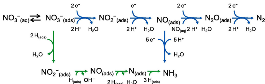
Fig. 2 The electron-mediated (blue arrow) and hydrogen atom-mediated (green arrow) pathways of the NO 3 RR. Reproduced with permission. 42 Copyright 2021, Elsevier B.V.
