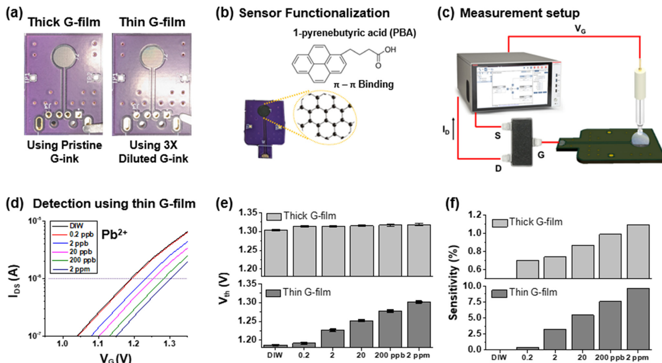
Fig. 3 Lead ion detection using the sensor PCB drop-casted by the graphene film (G-film). (a) Sensor PCBs bearing thick and thin G-films, deposited using pristine and 3× diluted G-inks, respectively. (b) Functionalization of the sensor PCBs for lead ion detection. (c) Detection setup using the sensor PCB, MOSFET, and analyzer. (d) Transfer curves of the MOSFET upon detection of lead ions ranging from 0.2 ppb to 2 ppb using thin G-film sensor. (e) and (f) Changes in threshold voltages ( V_{\text{th}} ) and sensitivity (%) with respect to lead ion concentrations using both thick and thin G-film sensors.
