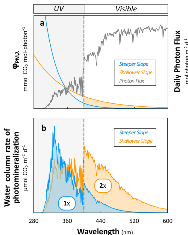
Fig. 1 Rates of DOM photomineralization in sunlit surface waters depend strongly on the wavelength-dependence of the AQY spectrum ( \phi_{PM,\lambda} ). (a) Two hypothetical \phi_{PM,\lambda} spectra (primary y-axis) are superimposed on a clear-sky solar spectrum from the Alaskan Arctic (secondary y-axis). The integrated \text{CO}_2 yields (areas under the curves) for both \phi_{PM,\lambda} curves are equal, but the shallower slope leads to greater photomineralization yields than the steeper slope in the visible region, which contains over 90% of the daily photon flux. (b) Water column rates of photomineralization calculated from the product of each of the two \phi_{PM,\lambda} spectra and the same photon flux spectrum shown in (a). Integrated water column rates of photomineralization (areas under the curves) calculated using the shallower \phi_{PM,\lambda} slope are double (2x) those calculated using the steeper \phi_{PM,\lambda} slope (1x).
