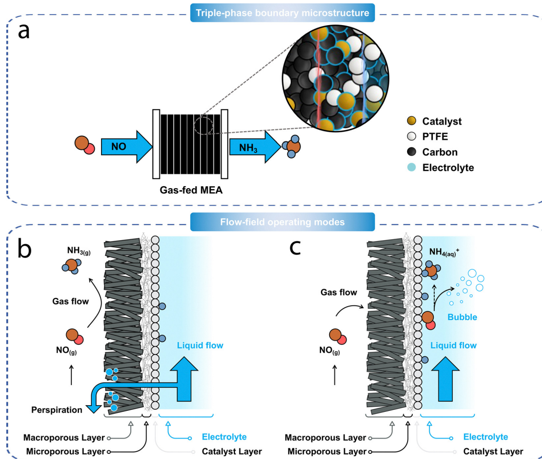
Fig. 12 (a) Microstructural rendering of the catalyst-ionomer-pore network at the triple-phase boundary. (b) Flow-by mode. \text{NO} -rich gas sweeps laterally across the GDE surface adjacent to the electrolyte, keeping gas saturation below \sim 40\% , suppressing flooding and nitrite/nitrate salt crystallisation, and allowing \text{NH}_3 to leave exclusively in the gas stream, so a simple condenser operating 5–10 K below cell temperature passively captures >95\% of the product while meeting occupational exposure limits. (c) Flow-through mode. Gas is driven through the porous electrode into the electrolyte channel, which shortens diffusion distances but raises the risk of electrolyte intrusion, precipitate clogging, and pressure-loss penalties familiar from \text{CO}_2 electrolyser systems.
