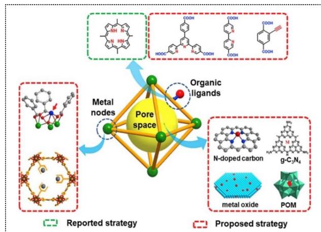
Fig. 11 Strategies for the production of ADMCs based on POMs. 32 Copyright 2019 Elsevier.
