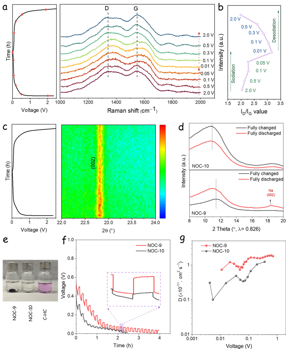
Fig. 4 Mechanistic study of the Na + storage process. (a) Ex situ Raman spectra from NOC-10 at 50 mA g -1 , corresponding to (b) I D /I G ratios. (c) In situ XRD patterns of NOC-10 at 50 mA g -1 . (d) The SXR patterns of NOCs were out with the fully charged and fully discharged states. (e) Optical photograph of samples discharged to 0.01 V vs. Na + /Na soaked in a 1% phenolphthalein ethanol solution for 5 min. (f) GITT curves at 300 mA g -1 . (g) Na + ions diffusion coefficient calculated from GITT.
