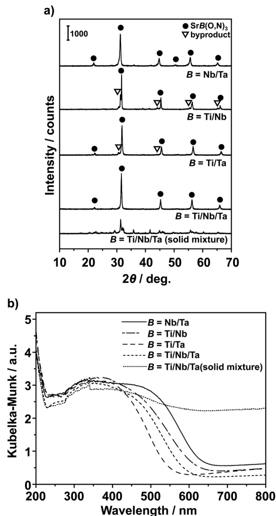
Fig. 4 (a) XRD patterns and (b) Kubelka–Munk-transformed UV-vis DRS of \text{SrBO}_2\text{N} ( B = \text{Nb}/\text{Ta} , \text{Ti}/\text{Nb} , \text{Ti}/\text{Ta} , and \text{Ti}/\text{Nb}/\text{Ta} ) prepared using sol-gel-derived precursors; data for \text{SrBO}_2\text{N} ( B = \text{Ti}/\text{Nb}/\text{Ta} ) prepared from a solid powder mixture of crystalline \text{TiO}_2 , \text{Nb}_2\text{O}_5 , and \text{Ta}_2\text{O}_5 is also shown for comparison.
