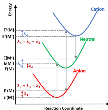
Fig. 8 Schematic energy profile of reorganization energy.
