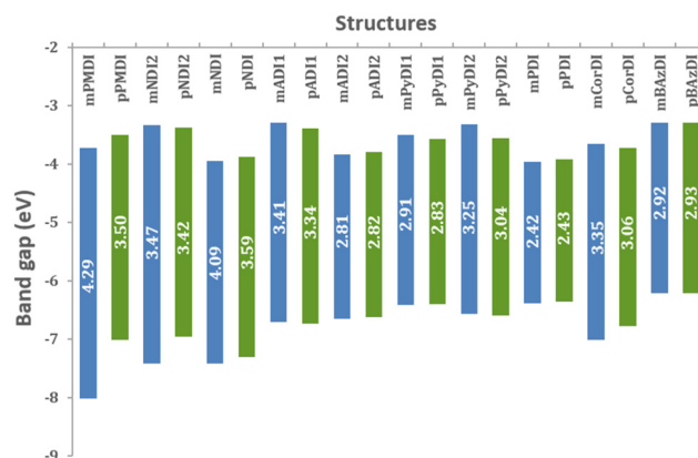
Fig. 3 Band gap energy of rylene diimides.
