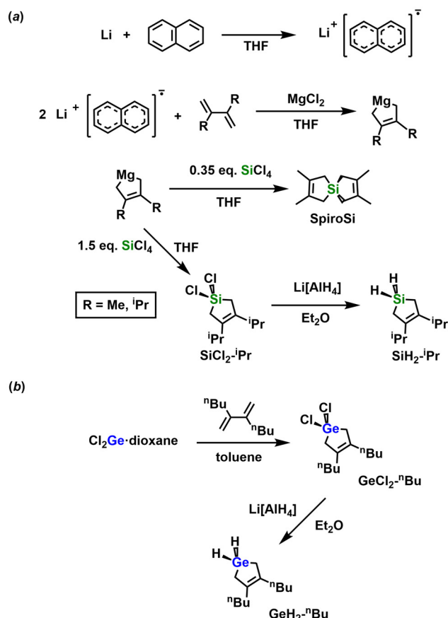
Scheme 1 (a) Synthesis of silaspiro-[4.4]-2,3,7,8-tetramethyl-2,7-nona-diene (SpiroSi) and 1,1-dihydro-3,4-di-iso-propylsilacyclopent-3-ene (SiH 2 -iPr); (b) synthesis of 1,1-dichloro-3,4-dibutylgermacyclopent-3-ene GeCl 2 - n Bu and 1,1-dihydro-3,4-dibutylgermacyclopent-3-ene GeH 2 - n Bu.
